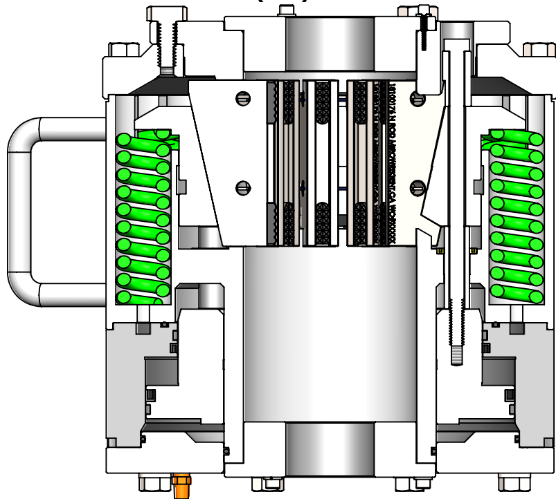
JAW SET / RETAINING RINGS / BUSHINGS
